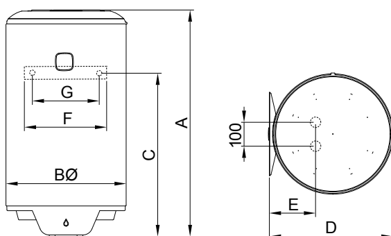
VERTICAL WALL-MOUNTED
