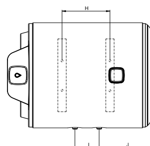
HORIZONTAL WALL-MOUNTED
